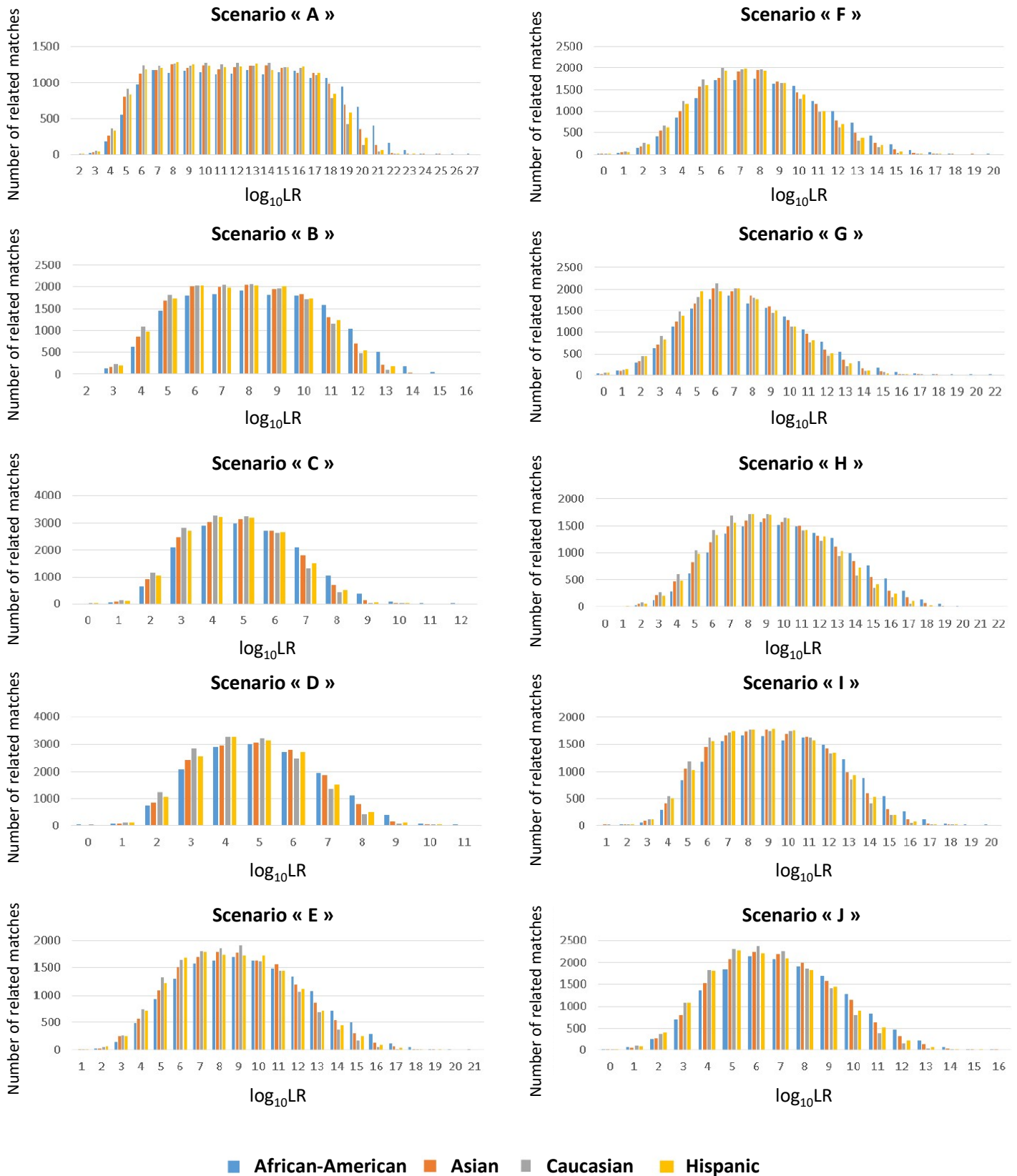
Figure S2 : \log_{10} LR Distributions of all the related matches obtained from the 10,000 pedigrees and for the 10 different scenarios. Four continental populations (African-American, Asian, Caucasian and Hispanic) were used and distribution curves showed an overlap and no differences in terms of mean of distribution and variance.
